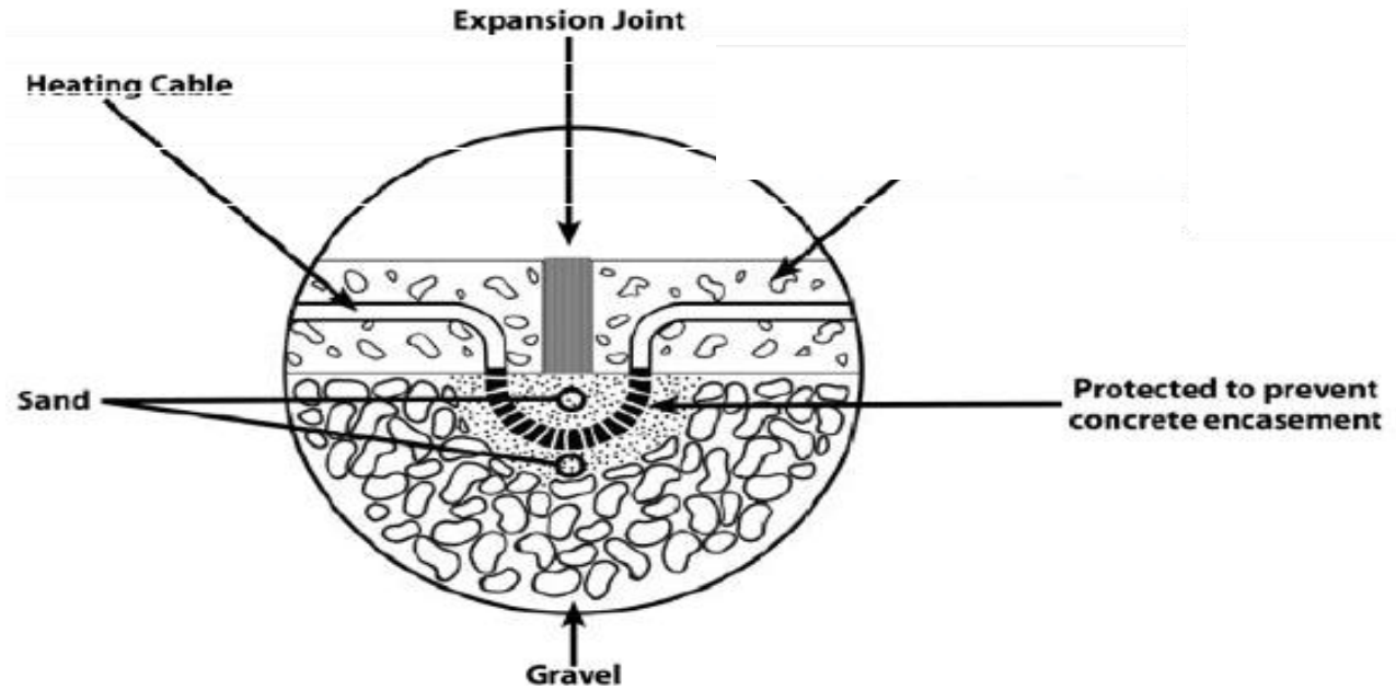
Figure 1: Expansion joint
